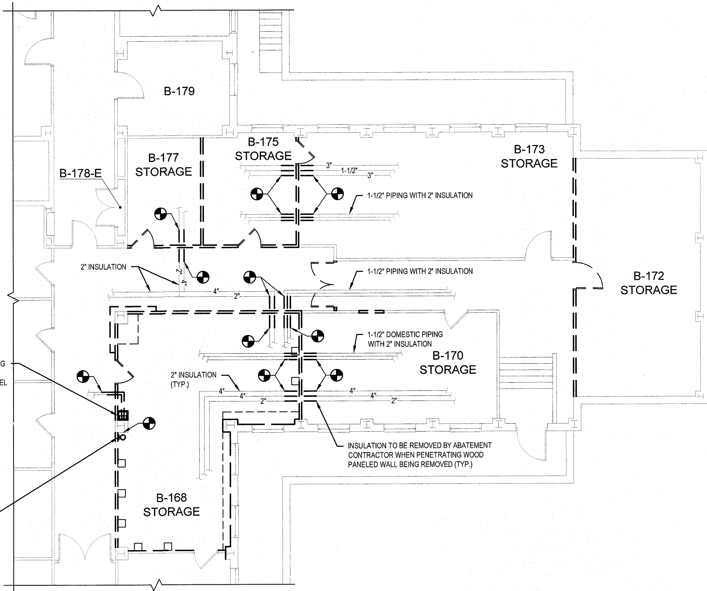
1 BASEMENT PLUMBING REMOVAL PLAN P-101 SCALE: 1/8" = 1'-0"
