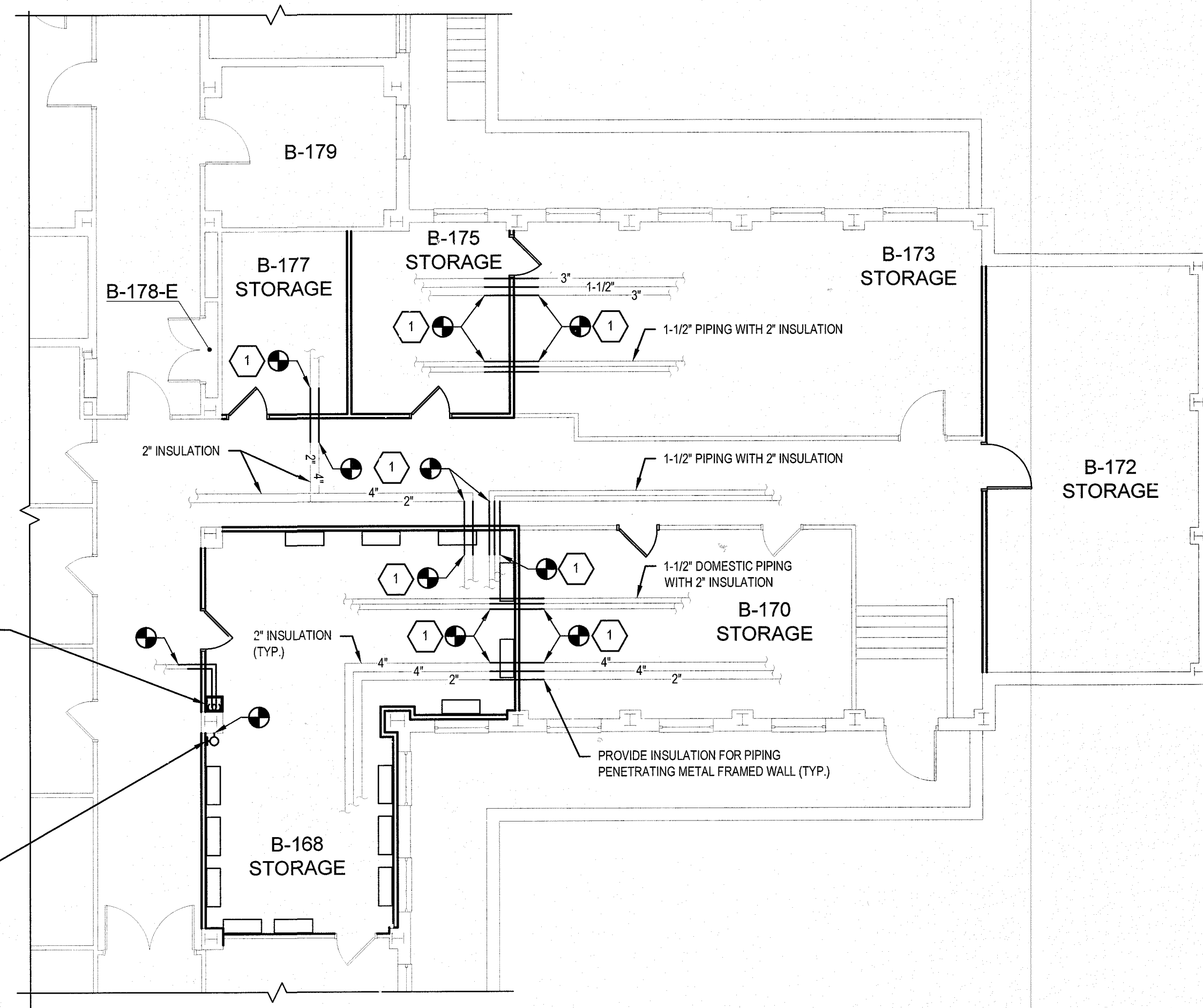
2 BASEMENT PLUMBING RENOVATION PLAN P-101 SCALE: 1/8" = 1'-0"
