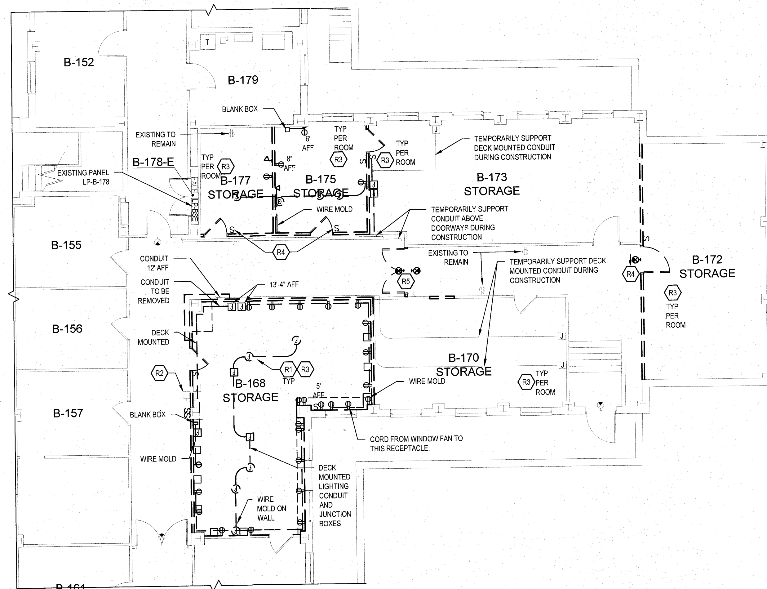
1 PARTIAL BASEMENT REMOVAL PLAN E-101 SCALE: 1/8" = 1'-0"
