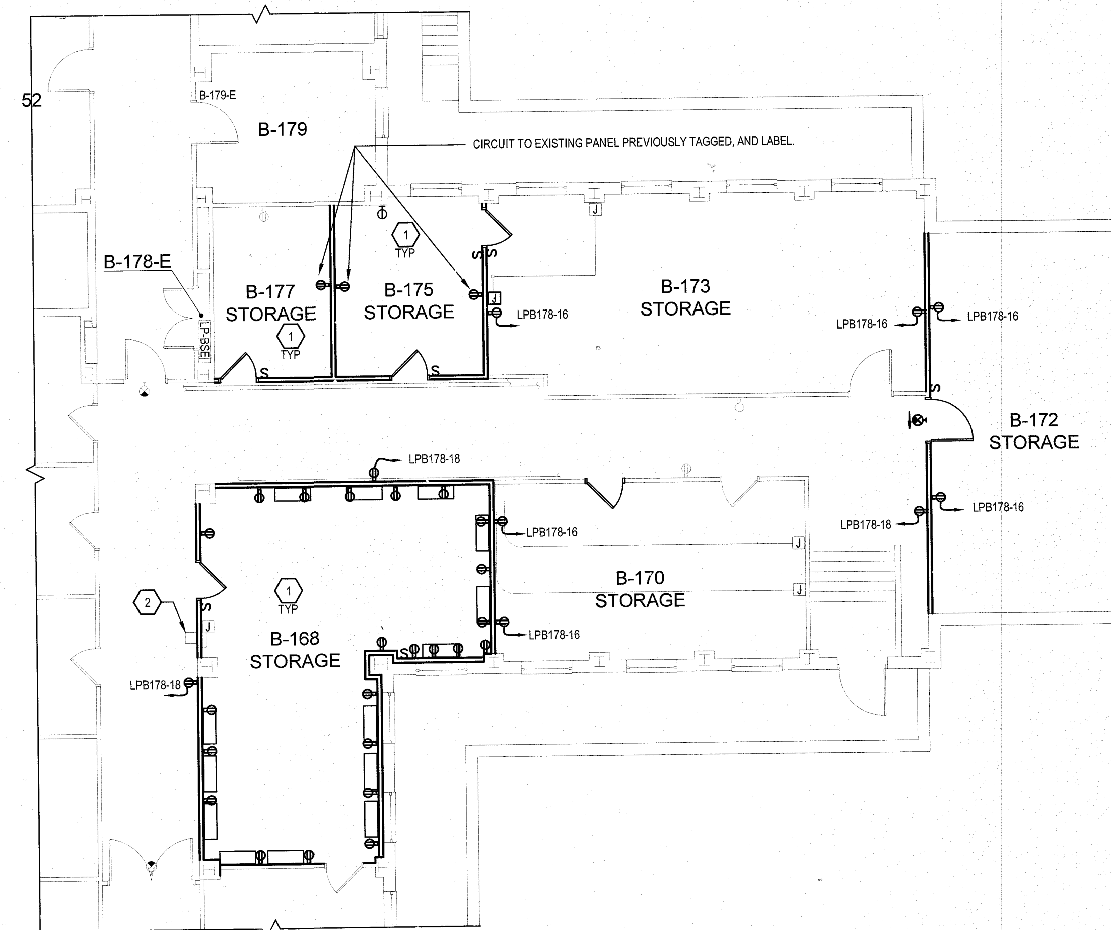
2 PARTIAL BASEMENT FLOOR PLAN E-101 SCALE: 1/8" = 1'-0"
